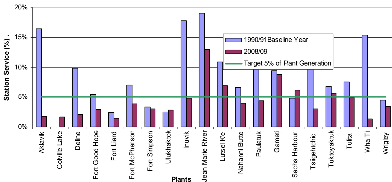
Figure 8: Station Service for Diesel Plants (excluding standby plants) for 1990/91 and 2008/09
