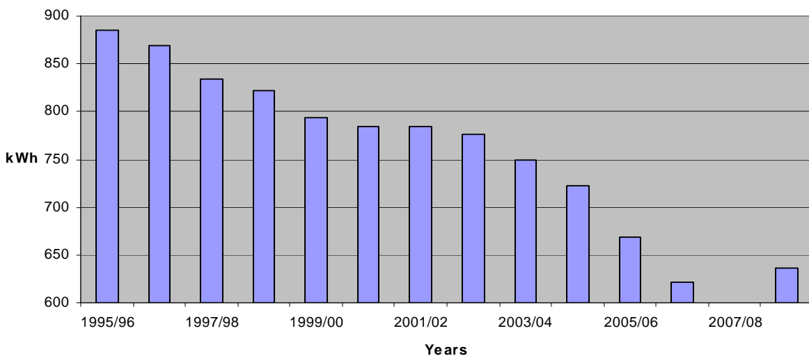
Figure 10: kWh per Streetlight per Year
