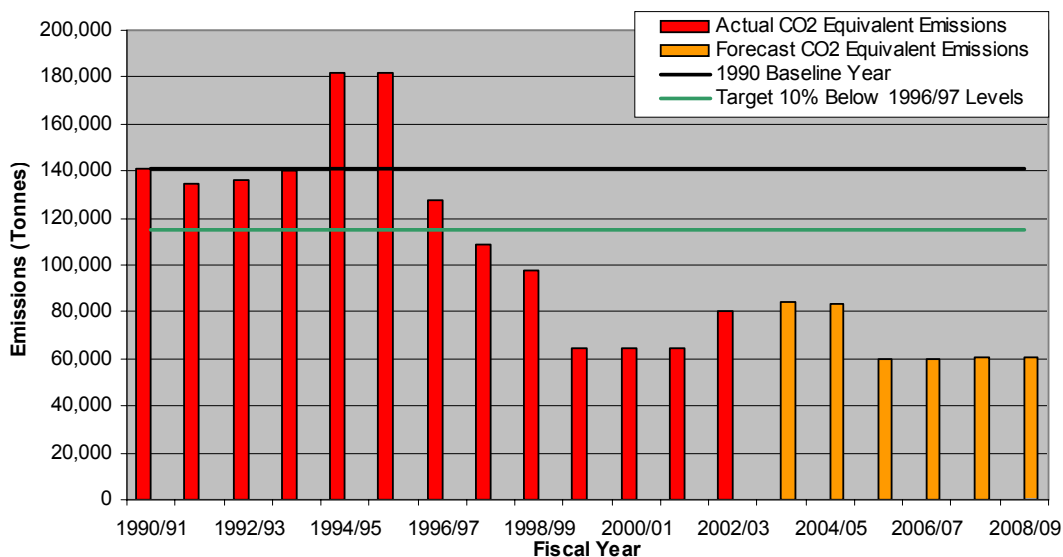
Figure 5: 2002/03 Forecast CO 2 Equivalent Emissions as a Product of Total Generation
