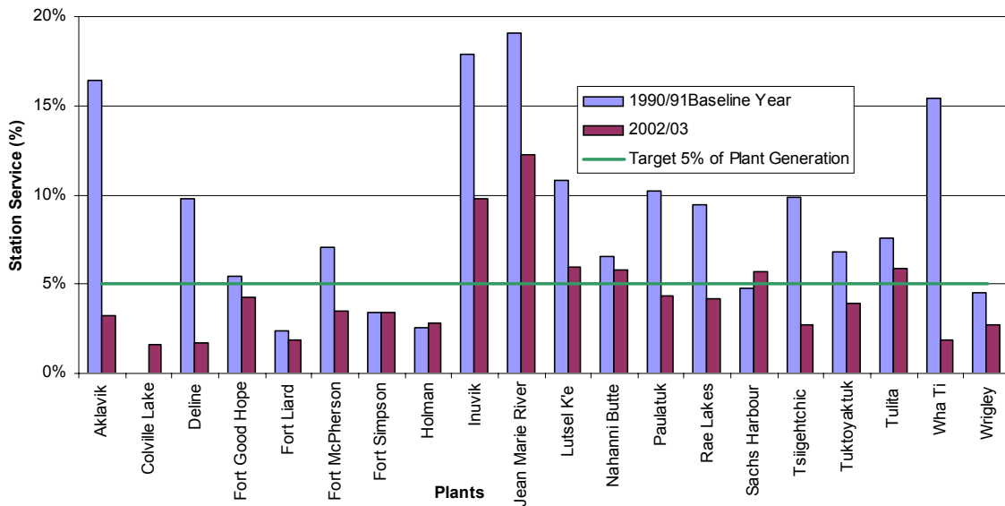
Figure 8: Station Service for Diesel Plants (excluding standby plants) for 1990/91 and 2002/03
